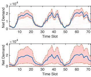
Figure 5: A sample illustration of net electricity demand as a function of interval prediction with 20% (top) and 80% (bottom) of the values
